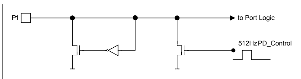
Fig.9: Port P1, P2 Input Pull Down
