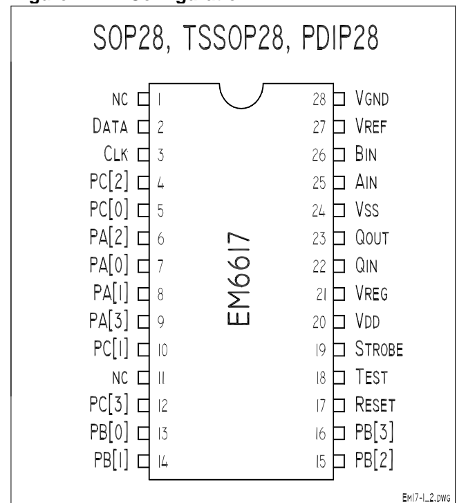
Figure 2. Pin Configuration
