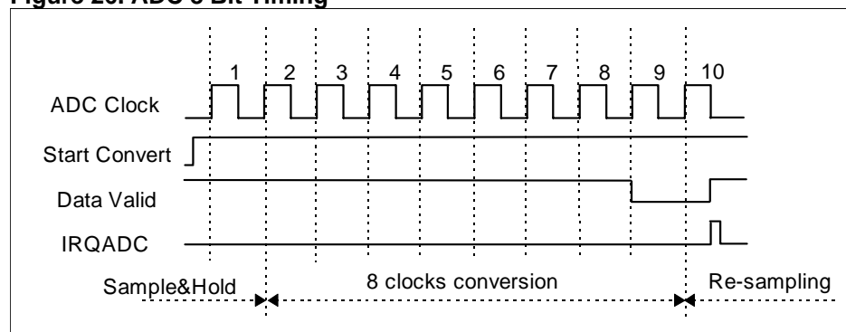
Figure 26. ADC 8 Bit Timing
