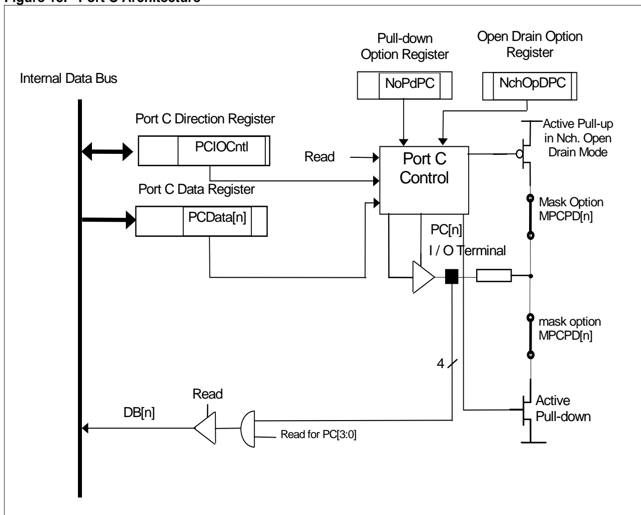
Figure 15. Port C Architecture
