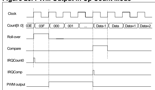
Figure 20. PWM Output in Up Count Mode
