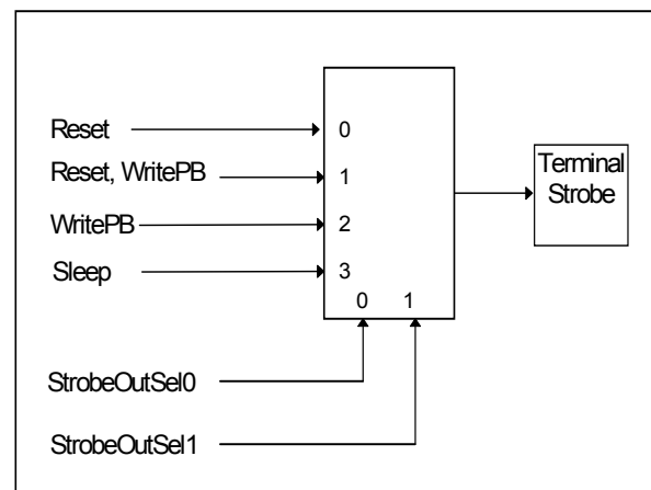
Figure 33 . Strobe Output
