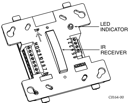
Figure 1A: Supervised Control Module
