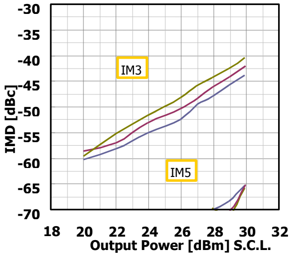
IMD Performance vs. Output Power by Case Temperature V_{DS}=10V I_{DS(DC)}=2200mA @5.9GHz
