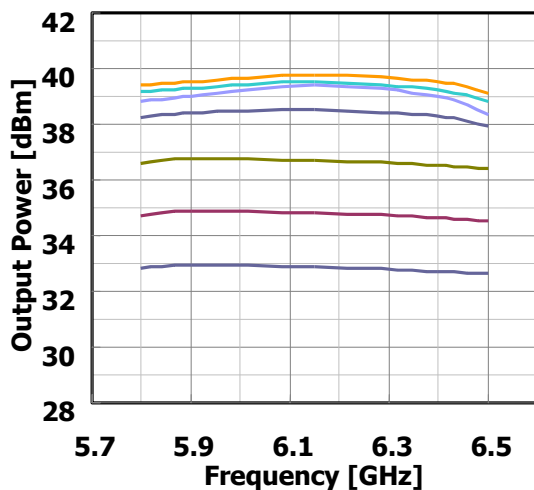
Output Power vs. Frequency V_{DS}=10V, I_{DS(DC)}=2200mA
