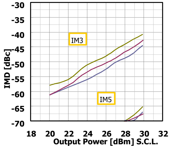
IMD Performance vs. Output Power by Case Temperature V_{DS}=10V I_{DS(DC)}=2200mA @6.15GHz
