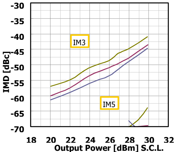
IMD Performance vs. Output Power by Case Temperature V_{DS}=10V I_{DS(DC)}=2200mA @6.4GHz
