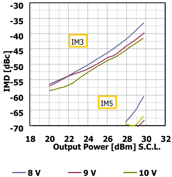
IMD Performance vs. Output Power by Drain Voltage I_{DS(DC)} = 2200\text{mA} @5.9GHz
