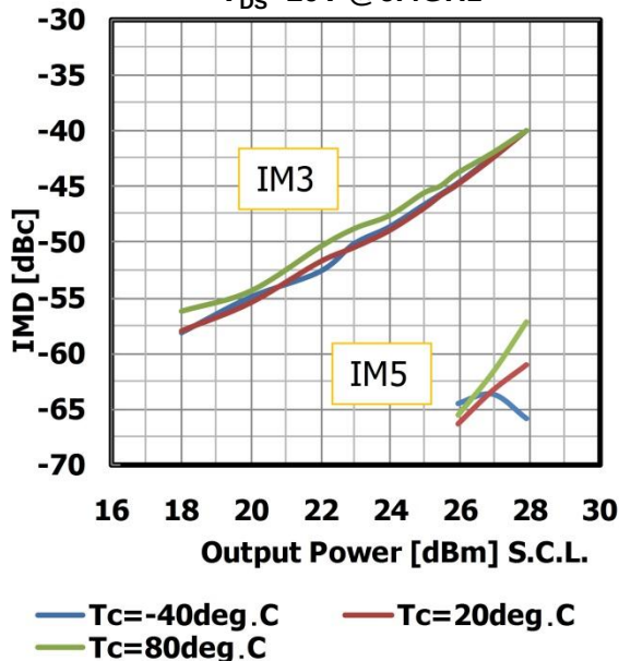
IMD Performance vs. Output Power by Temperature V_{DS}=10V @6.4GHz
