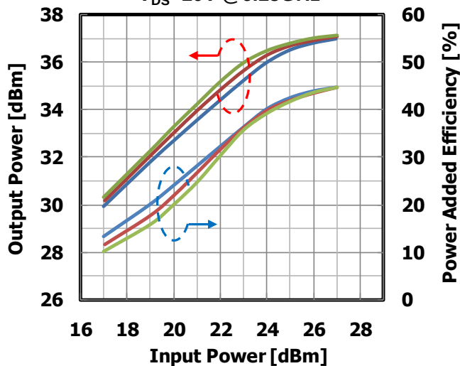
Input Power vs. Output Power, Power Added Efficiency by Quiescent Drain Current
