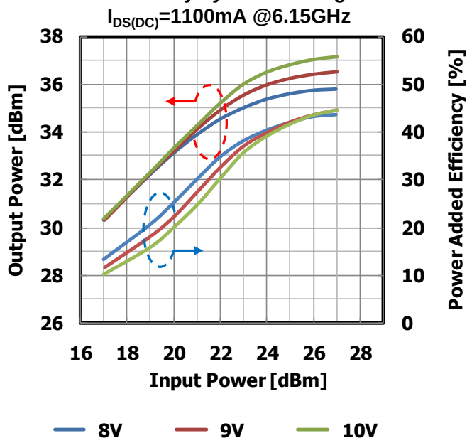
Input Power vs. Output Power, Power Added Efficiency by Drain Voltage I_{DS(DC)}=1100\text{mA} @6.15GHz
