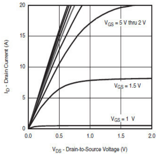
Output Characteristics
