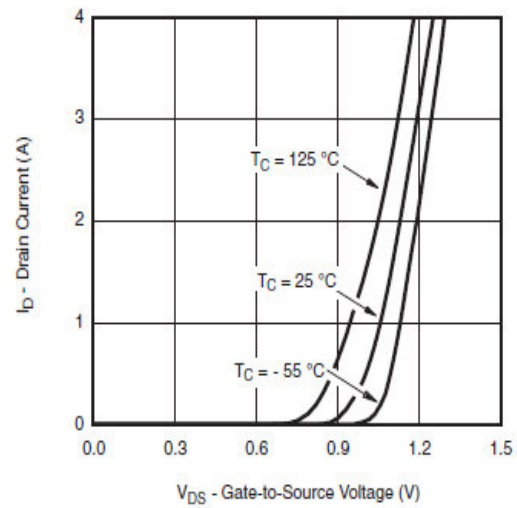
Transfer Characteristics
