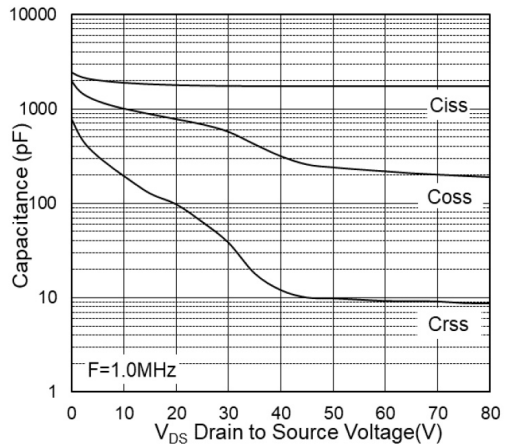
Fig.7 Capacitance
