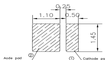
Soldering patterns
