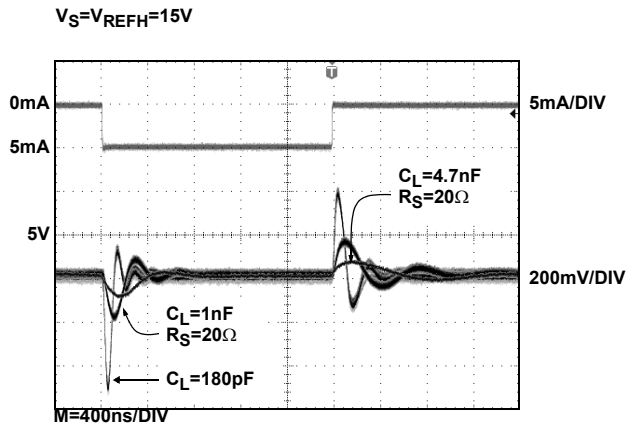
FIGURE 3. TRANSIENT LOAD REGULATION (SOURCING)
