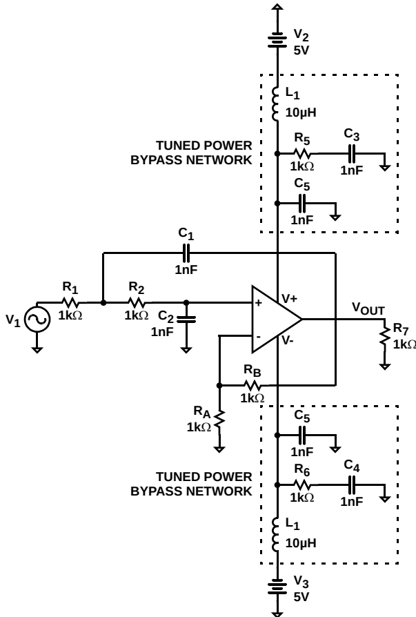
FIGURE 35. SULLEN KEY LOW PASS FILTER
