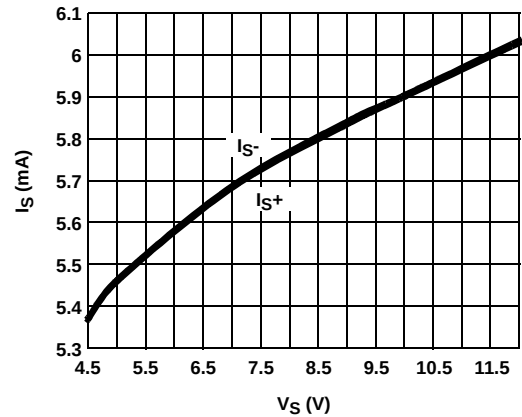
FIGURE 26. SUPPLY CURRENT vs SUPPLY VOLTAGE
