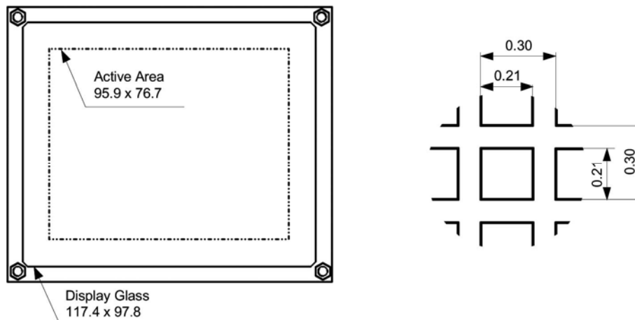
Fig 5. EL320.256-F6 and -FD6 display viewing area characteristics.
