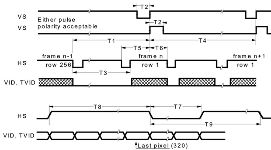
Figure 3. Timing Characteristics.
