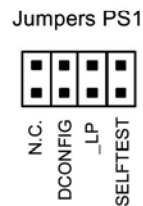
Fig 2. Input Connectors and Programmable Jumpers.
