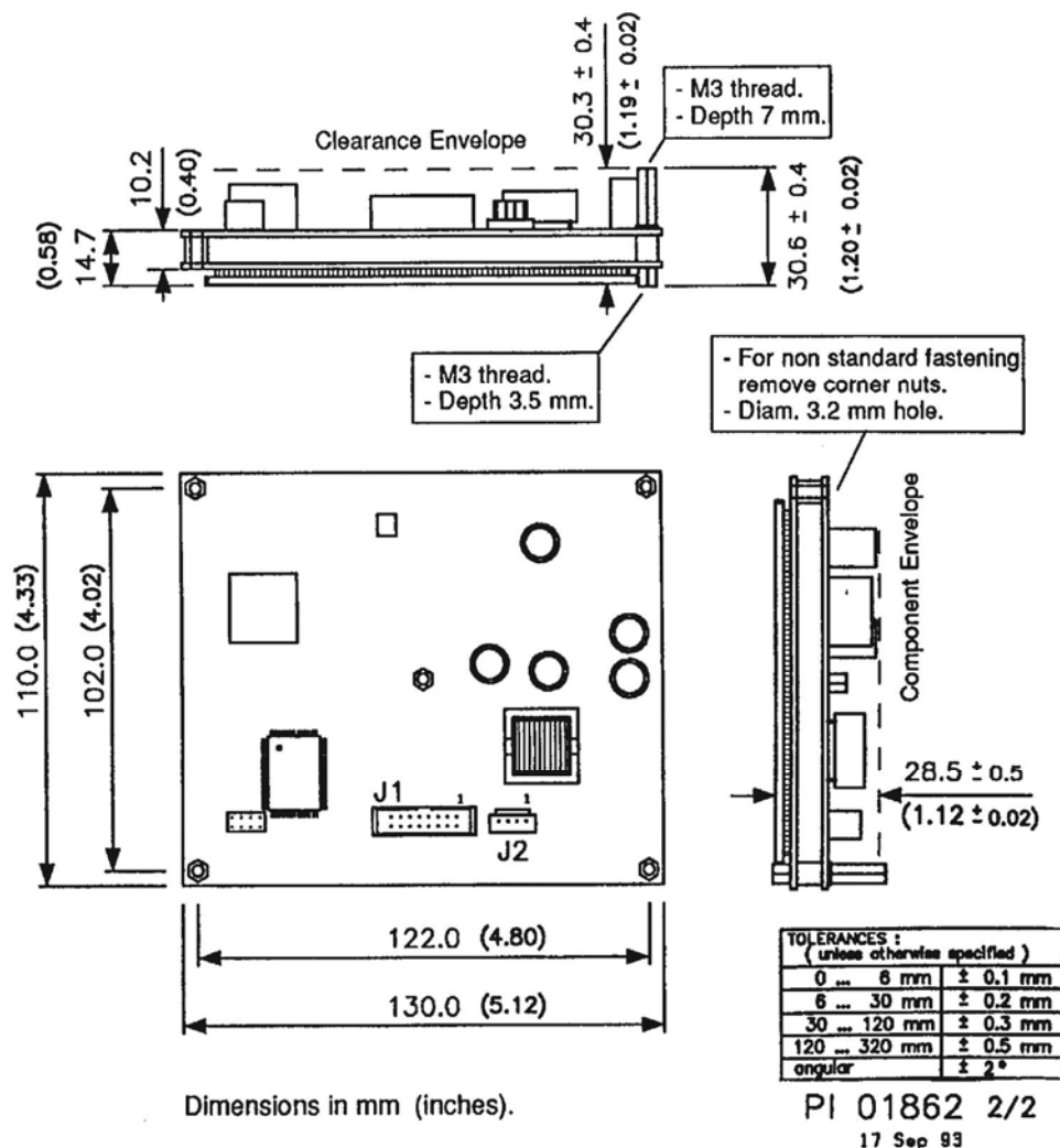
Fig 6. EL320.256-F6 and -FD6 display mechanical dimensions.
