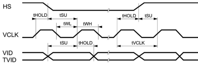
Figure 4. Setup and Hold Timing.
