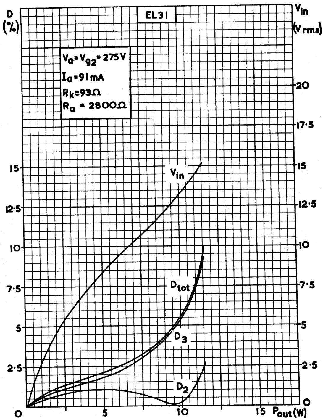
Fig. 4. Distortion curve for single valve at V_a = V_{g2} = 275 V. with simple feedback.
