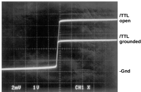
Input/Output Transfer Function - HYS Open
