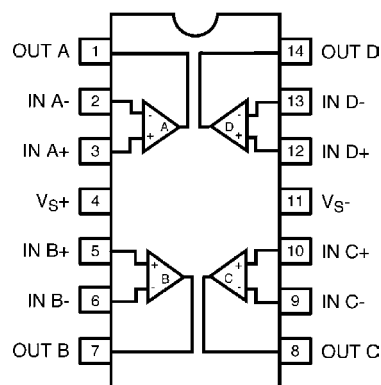
EL2470 (14-PIN SO, PDIP) TOP VIEW
