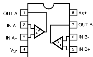
EL2270 (8-PIN SO, PDIP) TOP VIEW
