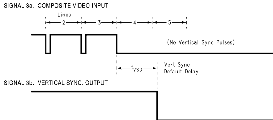
FIGURE 3. NON-STANDARD VERTICAL TIMING
