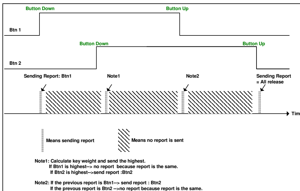
Fig. 11-2 Disable Multi-Finger Timing Diagram
