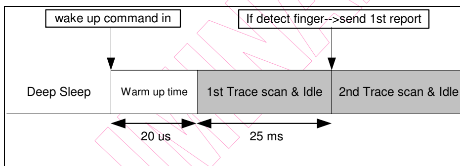
Fig. 7-2 Wake-up Timing from Deep Sleep Mode
