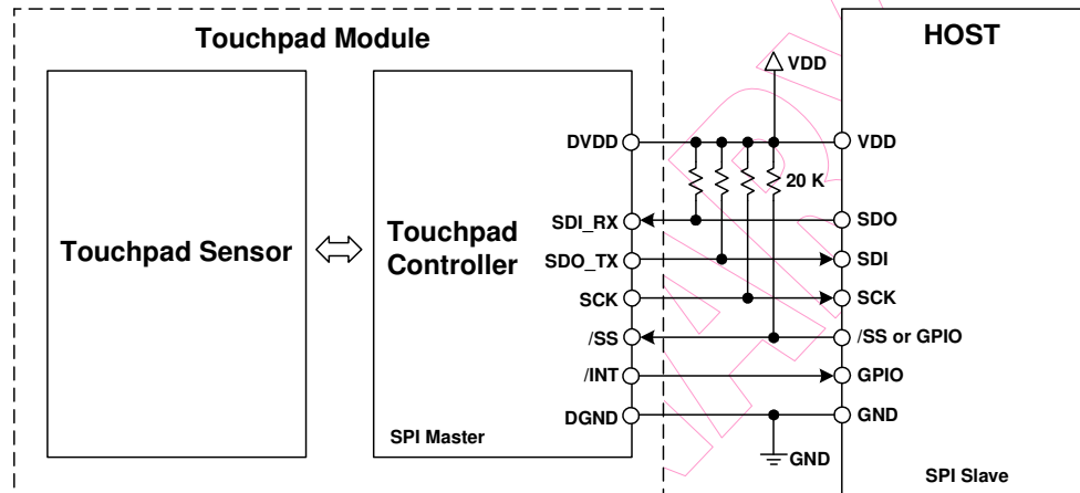
Fig. 4-3 System Block Diagram and SPI Interface
