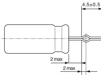
5 ≤ ØD ≤ 8 Leads bent open, shortened and formed EKS 09... (S = 5 mm)
