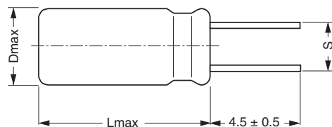
5 ≤ ØD ≤ 18 Shortened leads EKS 05... (S = 2 / 2.5 / 3.5 / 5 / 7.5 mm)
