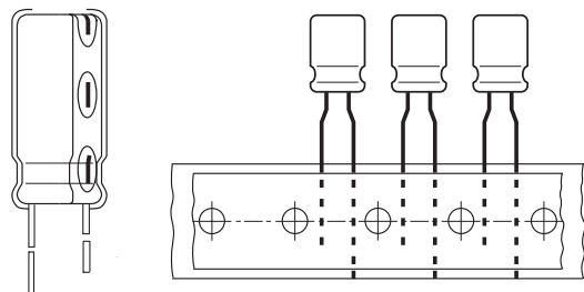
Component outlines.
