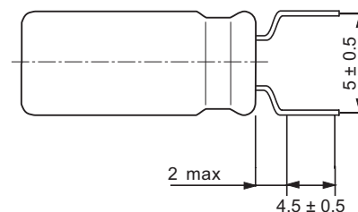
5 ≤ ØD ≤ 8 Leads bent open, shortened EKS 09... (S = 5 mm)
