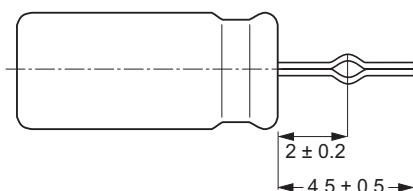
10 ≤ ØD ≤ 18 Leads shortened and formed EKS 06... (S = 5 / 7.5 mm)
