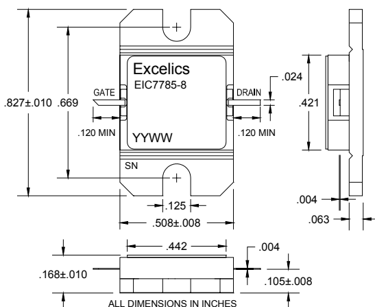
EIC7785-8 (Hermetic)
