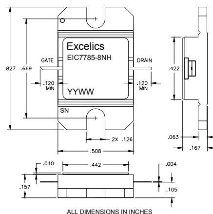
EIC7785-8NH (Non-Hermetic)
