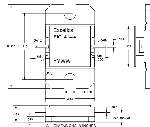
EIC1414-4 (Hermetic)
