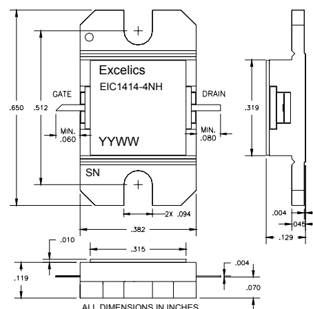
EIC1414-4NH (Non-Hermetic)
