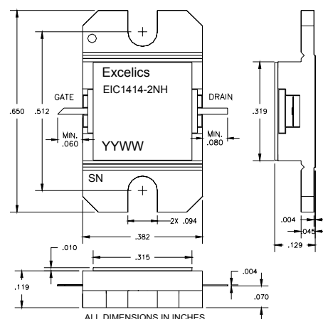
EIC1414-2NH (Non-Hermetic)
