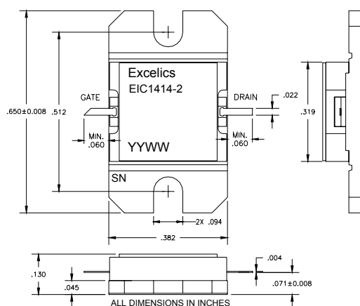
EIC1414-2 (Hermetic)
