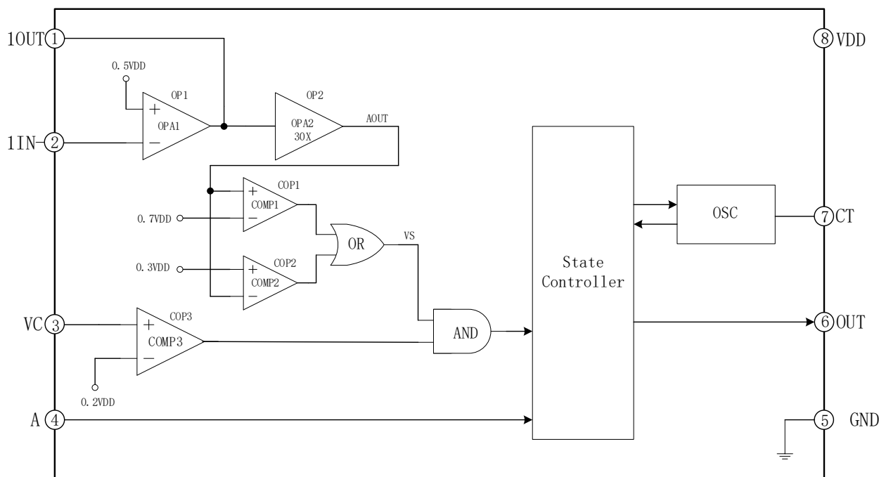
Figure 5.1 EG4002 block diagram
