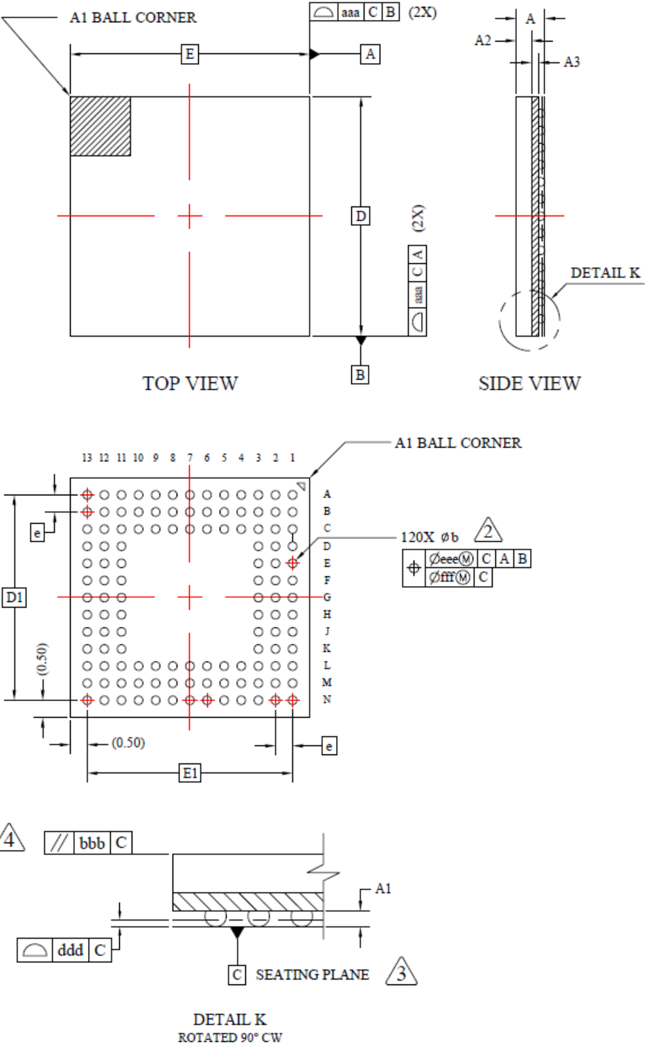
Figure 6.1. BGA120 Package Drawing
