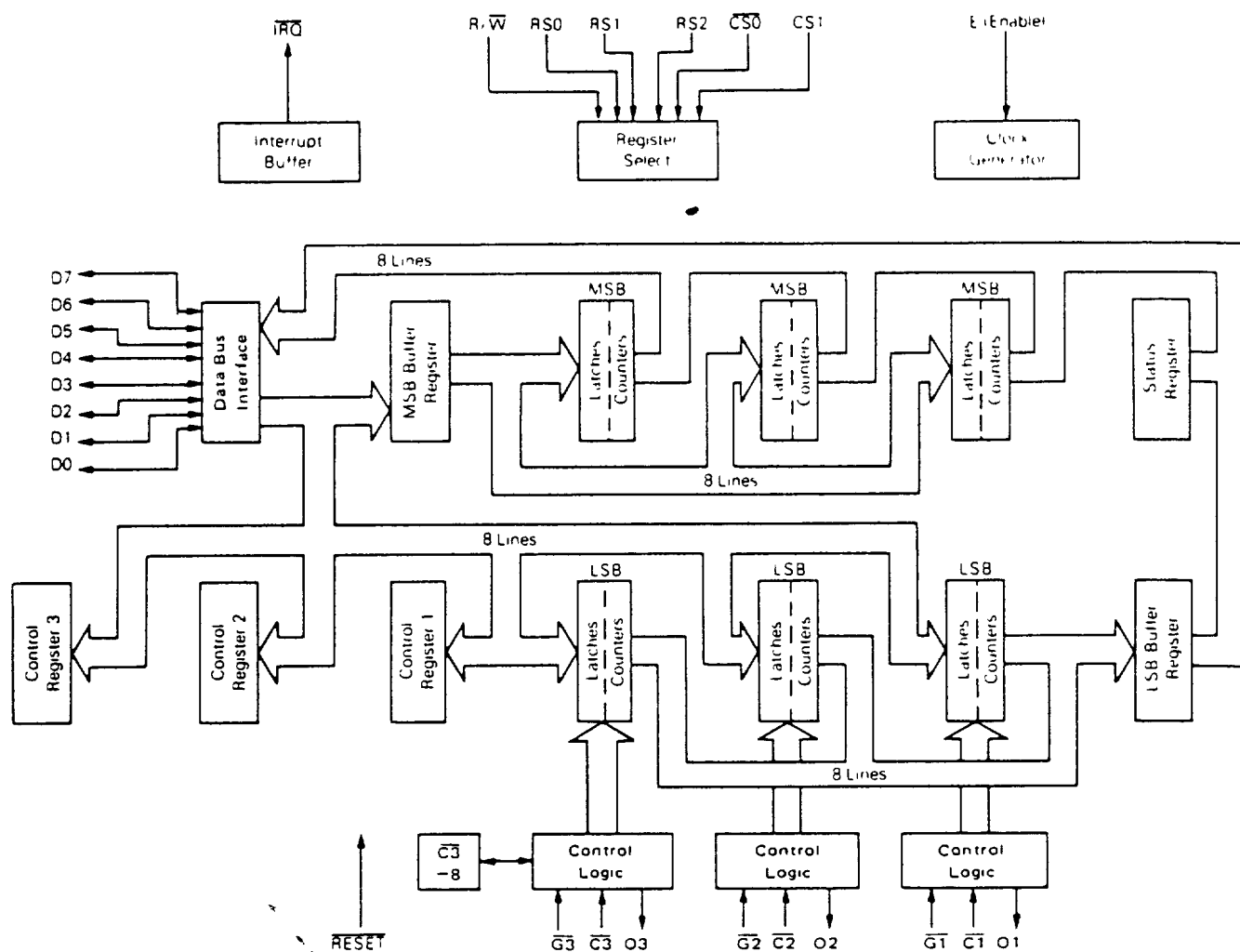
FIGURE 2 — BLOCK DIAGRAM
