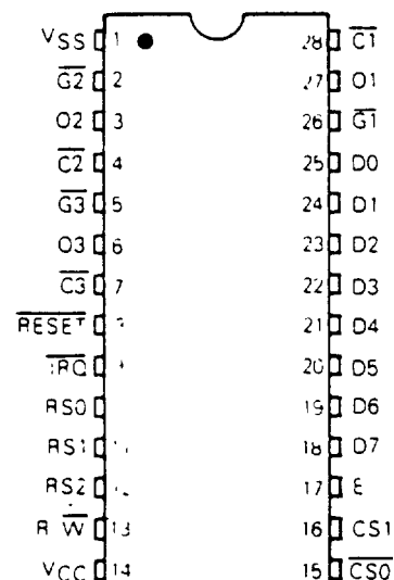
FIGURE 1 — PIN ASSIGNMENT
