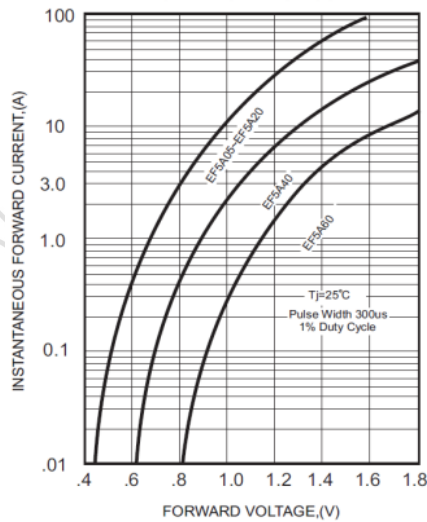
FIG.3-TYPICAL FORWARD CHARACTERISTICS
