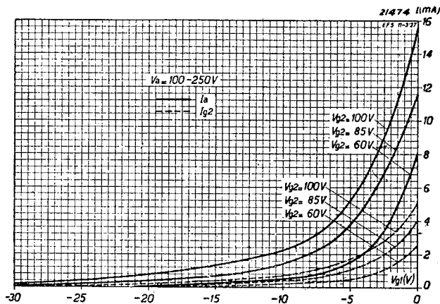
Fig. 3 Anode current and screen current as a function of the grid bias, for different values of screen potential, at 250 V anode. The curves also apply as an approximation to anode voltages of 100–250 V.
