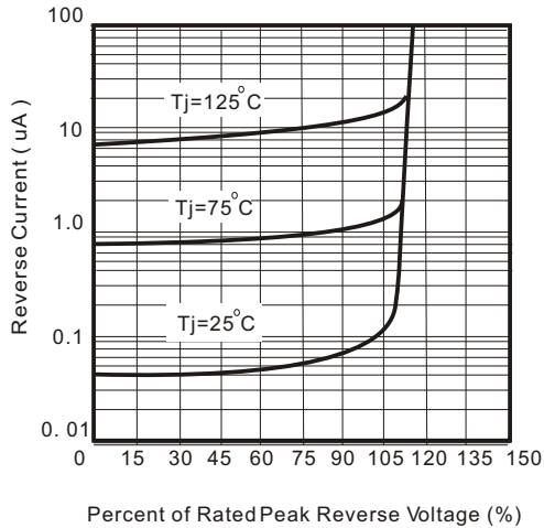
Fig. 1 - Reverse Characteristics
