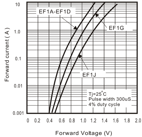
Fig.2 - Forward Characteristics
