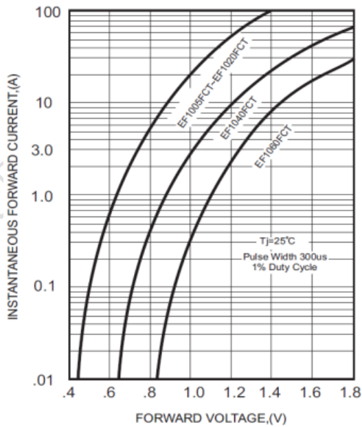
FIG.3-TYPICAL FORWARD CHARACTERISTICS
