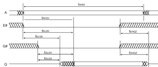
FIG. 2 TIMING WAVEFORM — READ CYCLE
