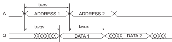
FIG. 2 TIMING WAVEFORM — READ CYCLE
