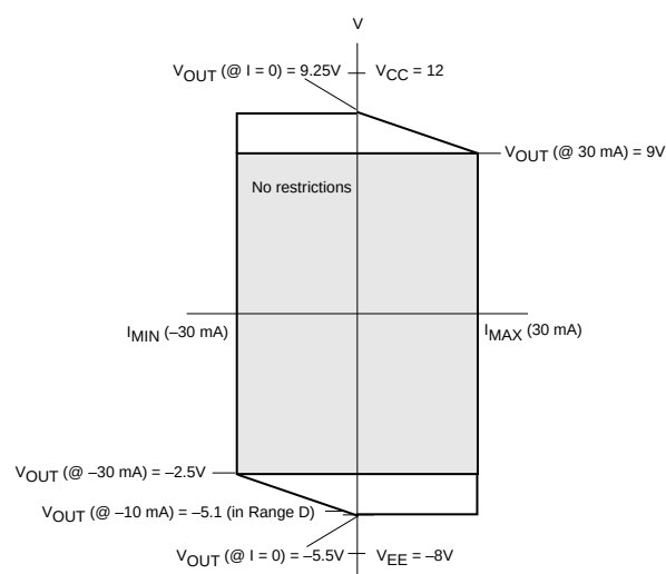
Figure 1. PMU Functionality
