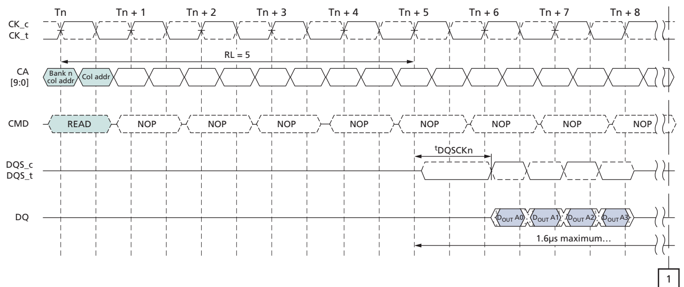
Figure 27: t_{DQSKDM} Timing
