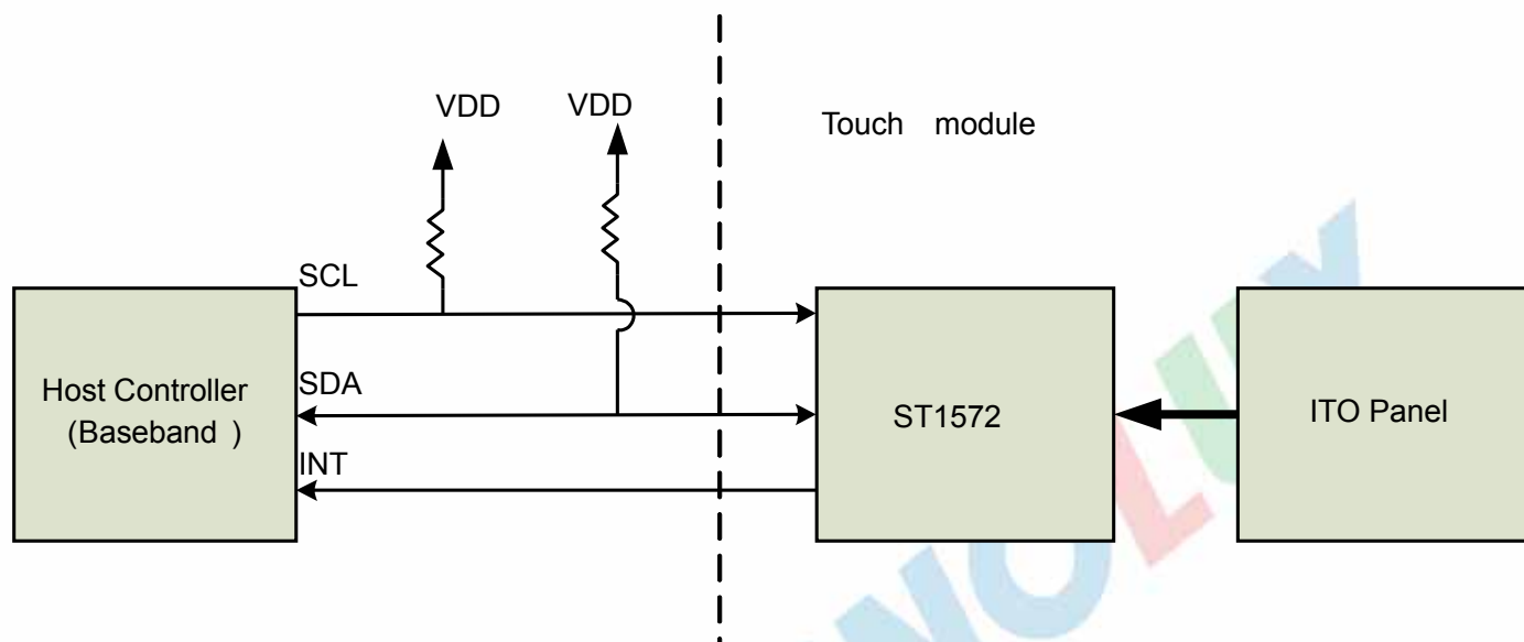
Figure 3 Touch module diagram
