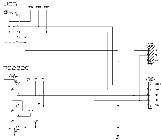
PWB assembly CONTROL (CC9XM2)
