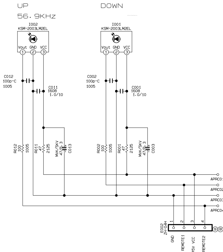
PWB assembly REMOTE (CC9XM2)
