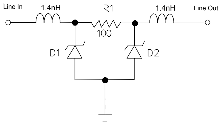
Figure 1 - EClamp2378P Spice Model
