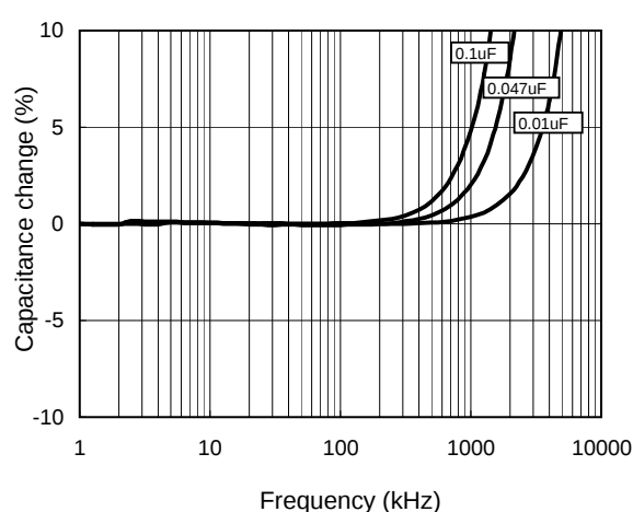
Frequency Characteristics
