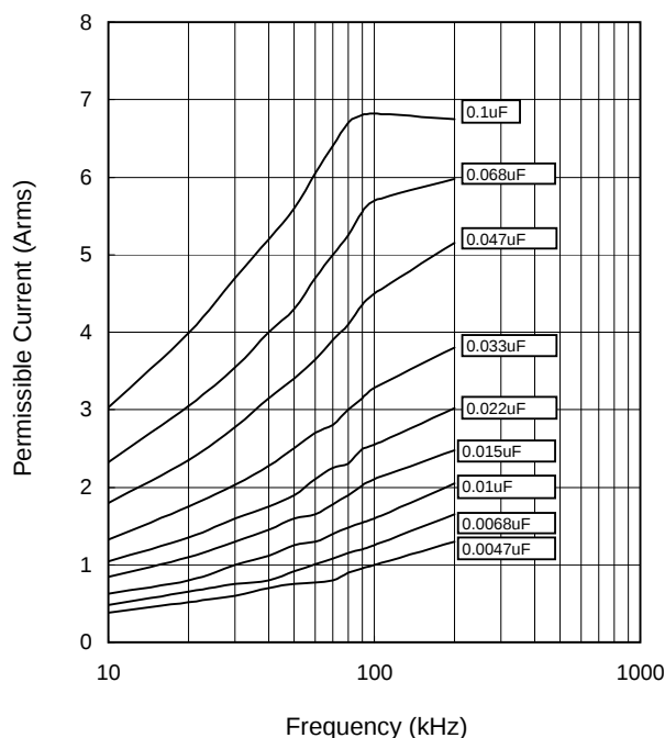
Permissible Current
