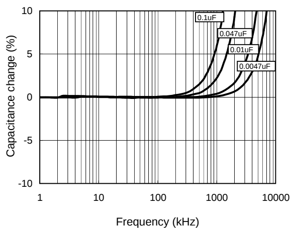
Frequency Characteristics
