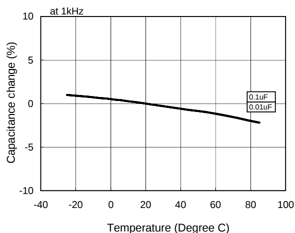
Temperature Characteristics
