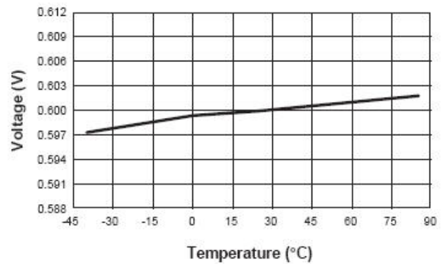
V_{FB} vs. Temperature ( V_{IN} = 3.6V ; V_{OUT} = 1.8V ; I_{LOAD} = 0mA )
