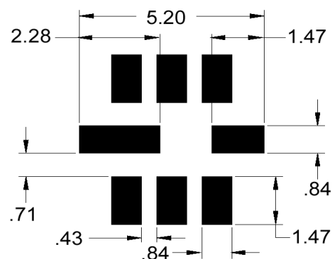
Figure 2) Suggested Land Pattern
