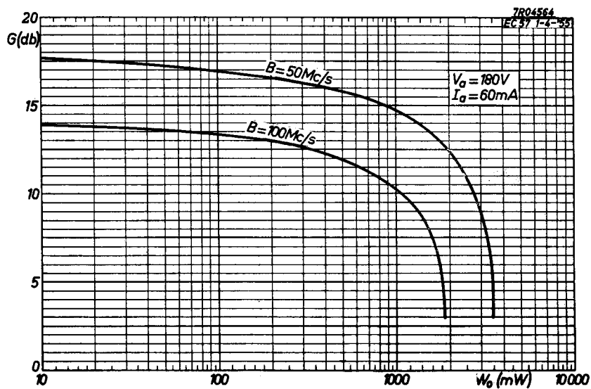
Fig. 48. Power gain G of the EC 57 as a function of the output power W_o with the bandwidth B as parameter at an anode current I_a = 60 mA.
