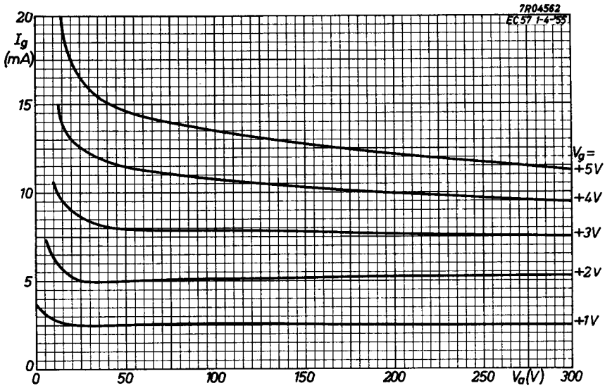
Fig. 45. I_g/V_a characteristics of the EC 57.
