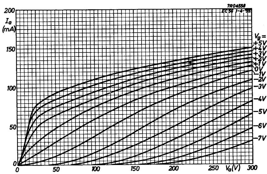
Fig. 43. I_a/V_a characteristics of the EC 56.
