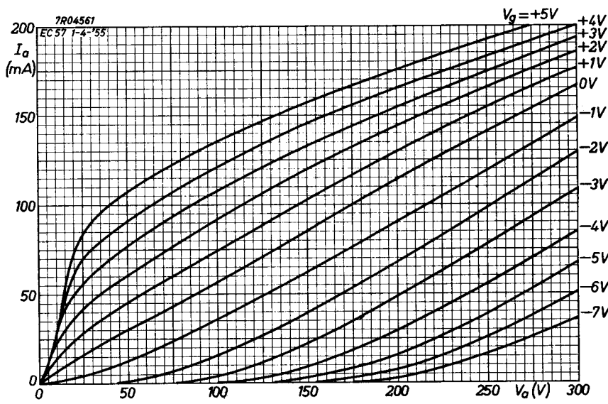
Fig. 44. I_a/V_a characteristics of the EC 57.
