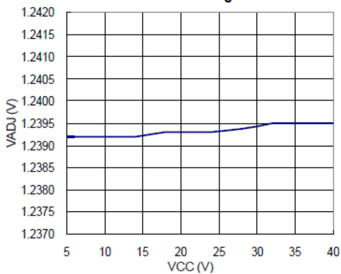
Reference Voltage vs. VCC
