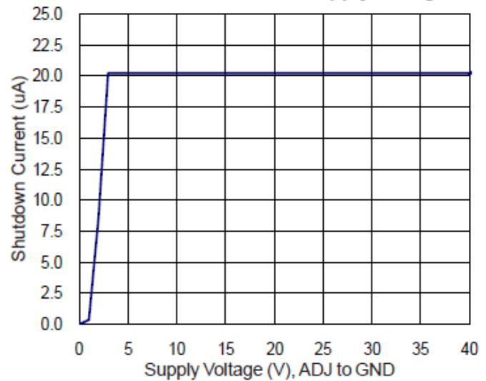
Shutdown Current vs. Supply Voltage
