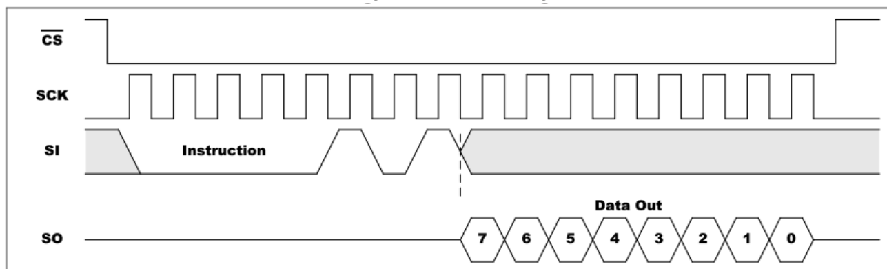
Figure 4. RDSR Timing
