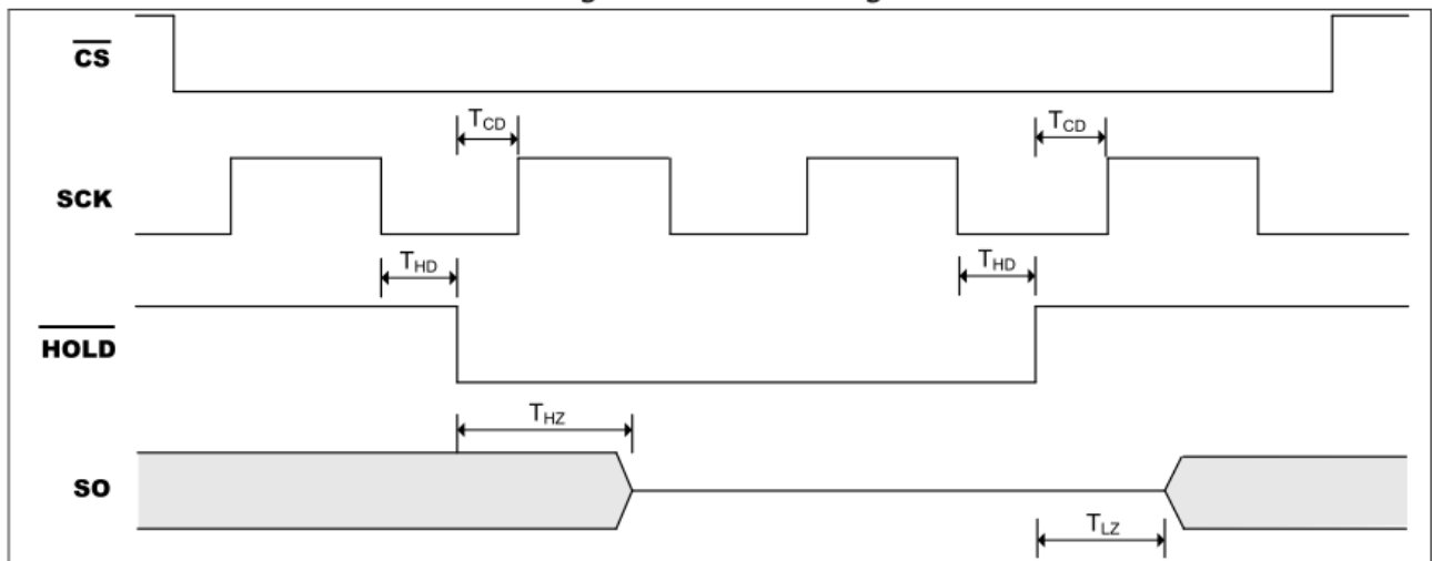
Figure 8. HOLD Timing
