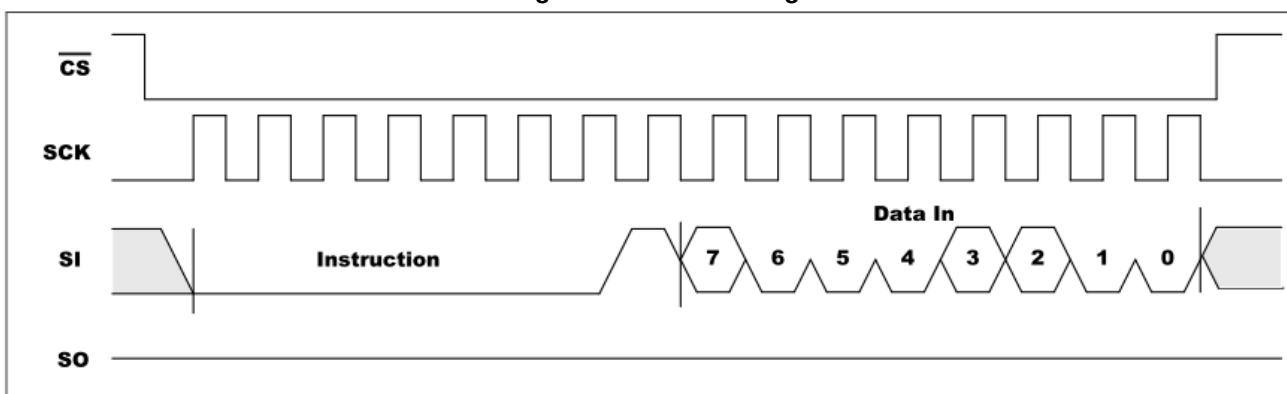
Figure 5. WRSR Timing
