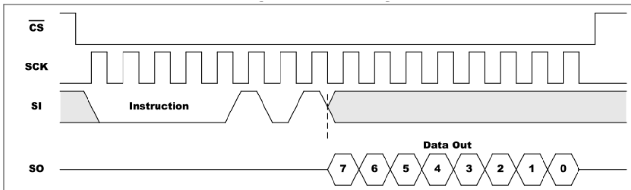
Figure 4. RDSR Timing
