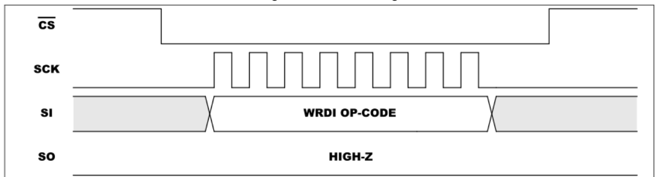
Figure 3. WRDI Timing
