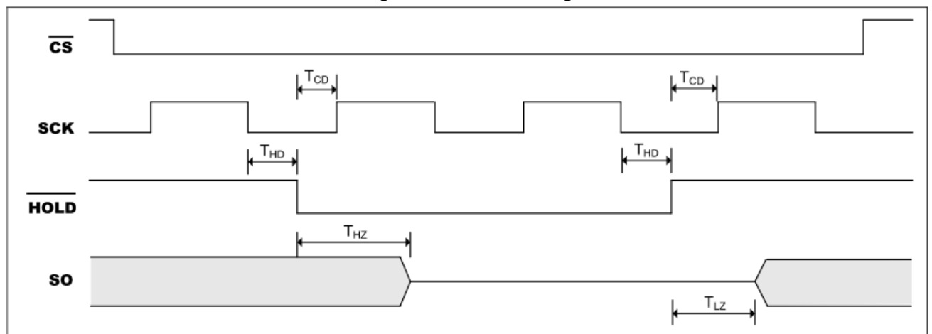
Figure 12. HOLD Timing
