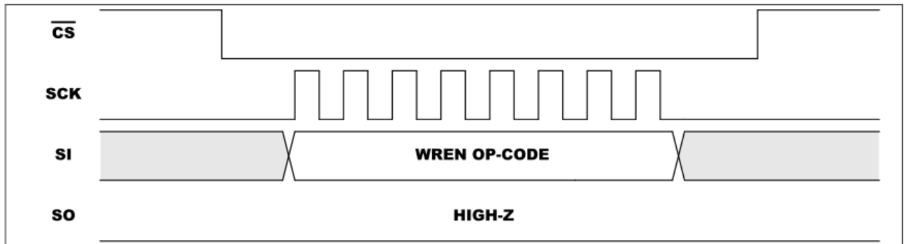
Figure 2. WREN Timing
