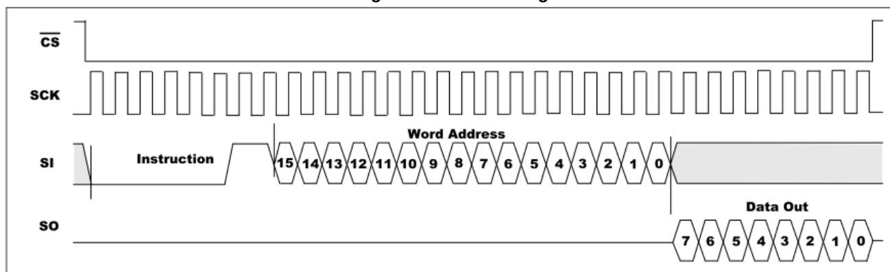
Figure 6. READ Timing
