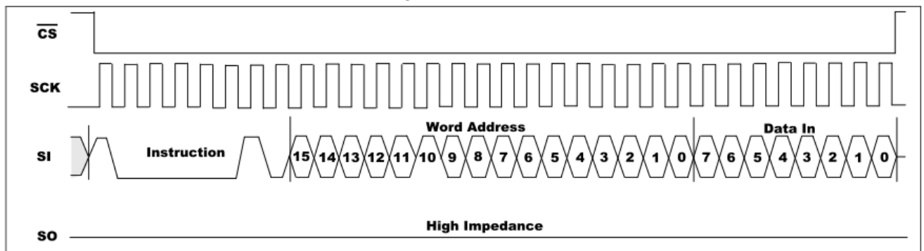
Figure 11. Lock ID
