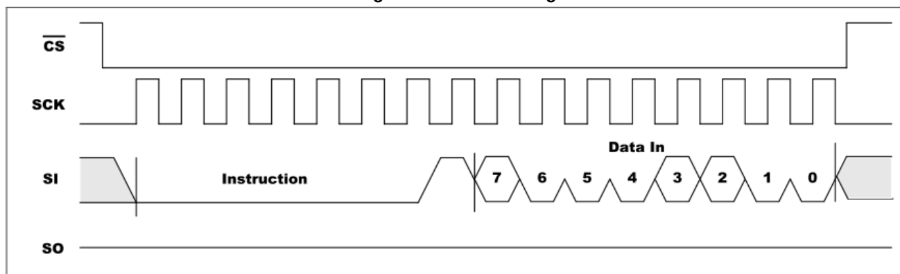
Figure 5. WRSR Timing
