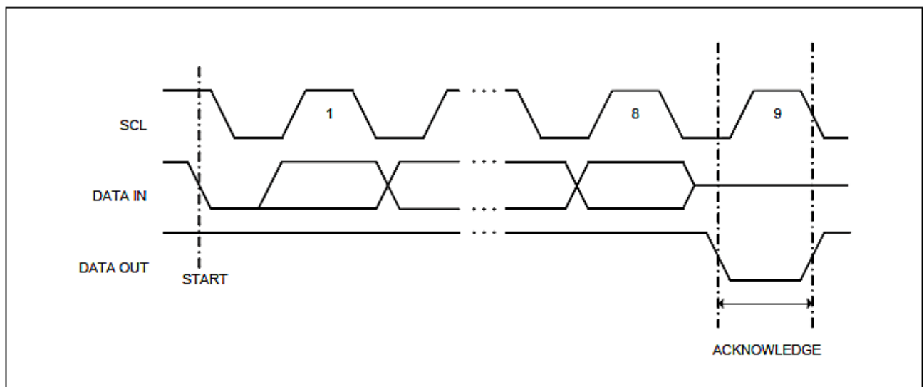
Figure 3: Output Acknowledge
