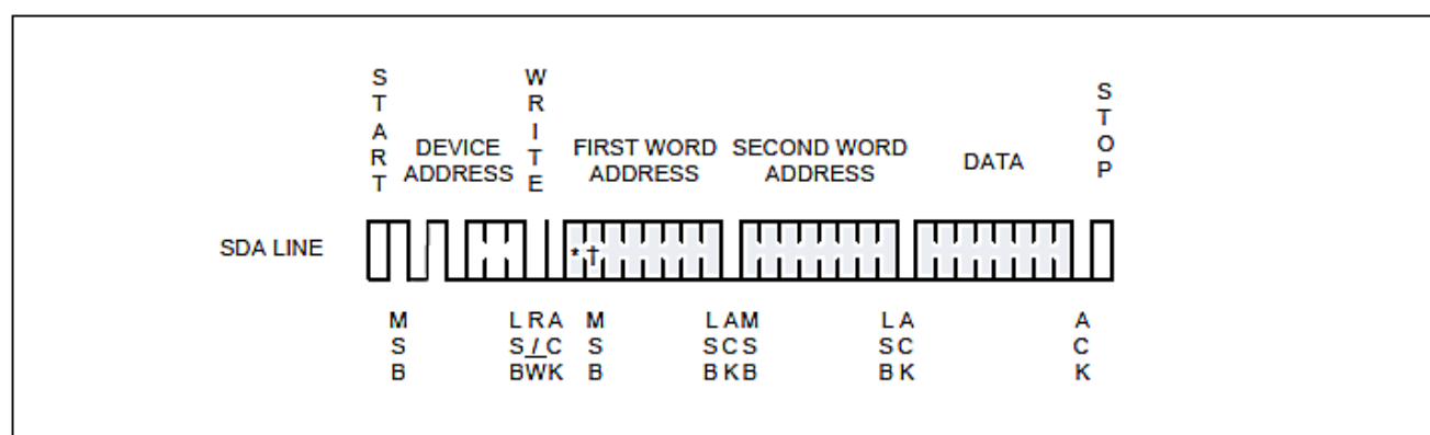
Figure 5: Byte Write
