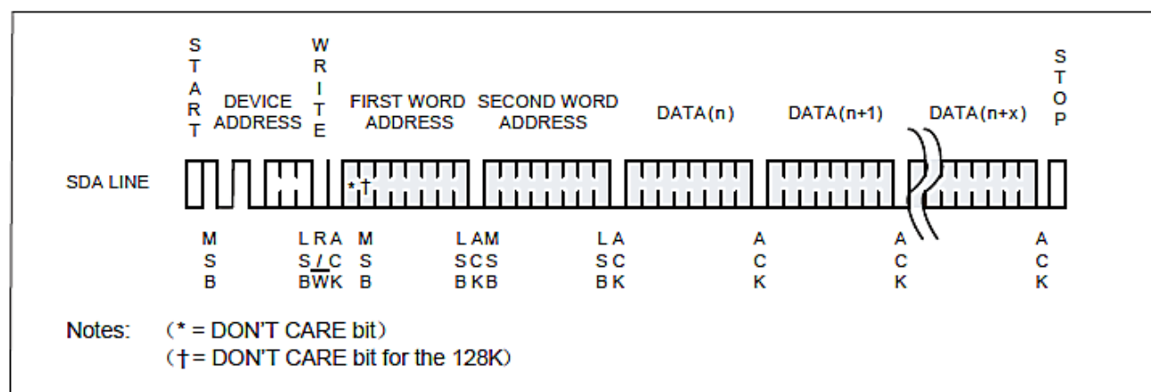
Figure 6: Page Write
