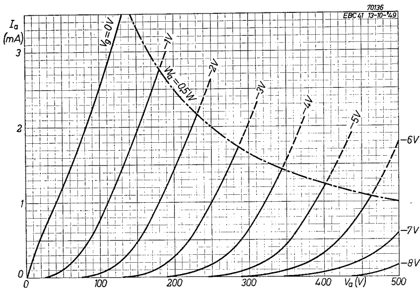
Fig. 5 I_a/V_a characteristics of the EBC 41 for different values of the grid bias V_g . The dotted line indicates the maximum permissible anode dissipation.
