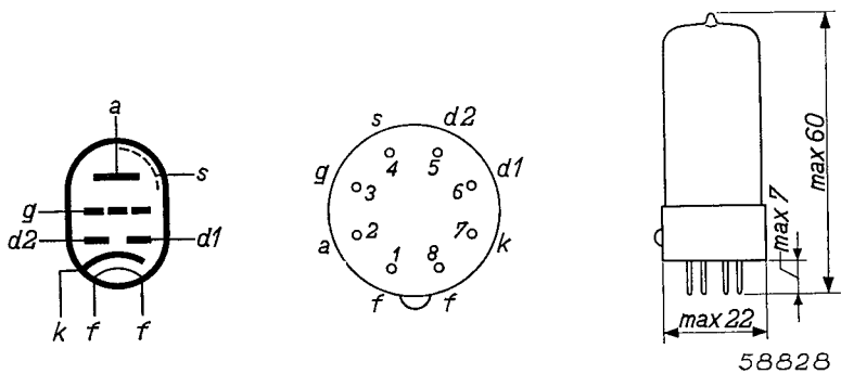
Fig. 2 Electrode arrangement, electrode connections and maximum dimensions of the EBC 41 (dimensions in mm).
