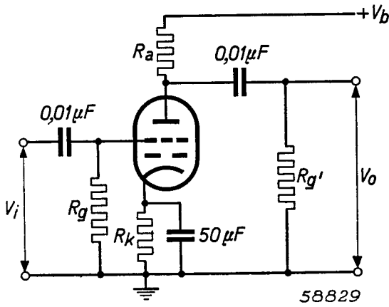
Fig. 3 The EBC 41 used as A.F. amplifier with resistance coupling. R'_g represents the grid leak of the next valve.
