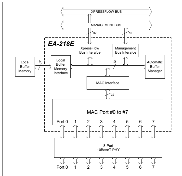
Block Diagram –
