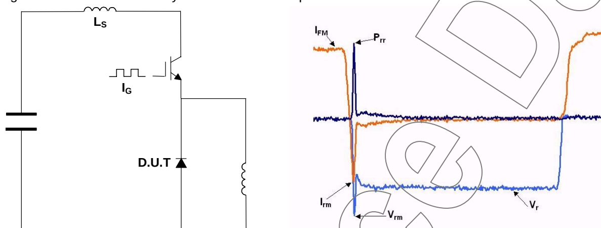
Diagram 1 – Reverse Recovery test circuit and sample waveform
