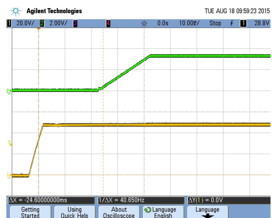
Startup Delay (Vin = 48V, Iout = 60A, Cload = 1000uF, Ta = +25°C) Ch1 = Vin, Ch2 = Vout
