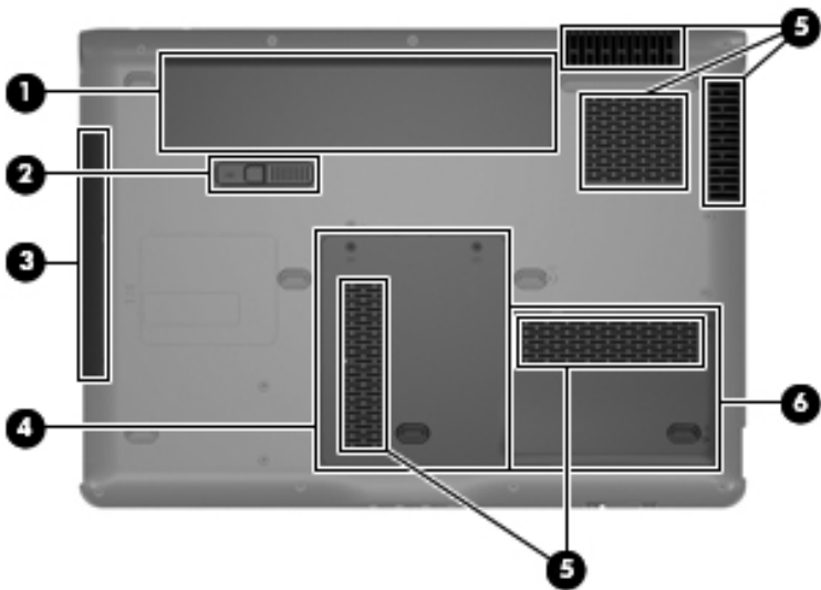
Bottom Components
