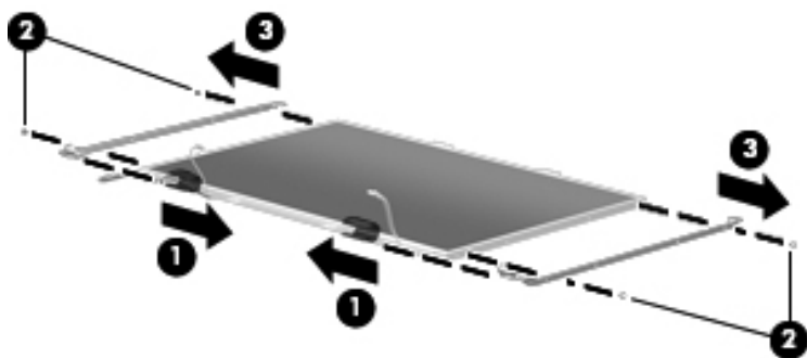
Removing the Display Hinges
