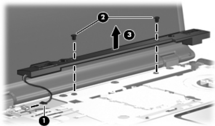
Removing the Speaker Assembly
