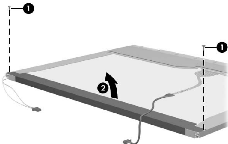
Removing the Backlight Cover
