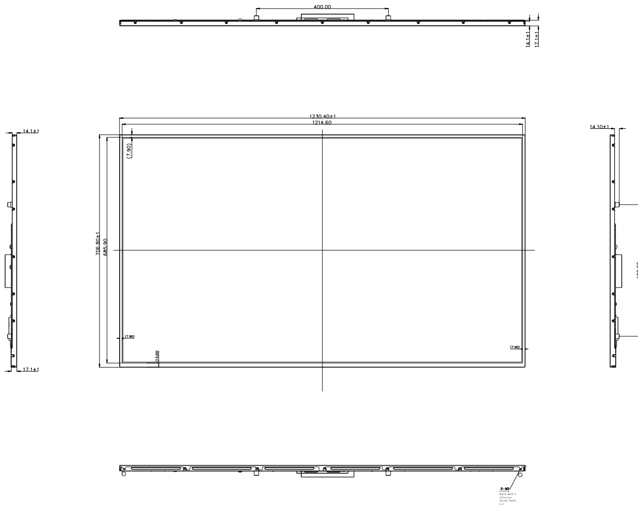
TFT-LCD Module Outline Dimensions ( Front View )
