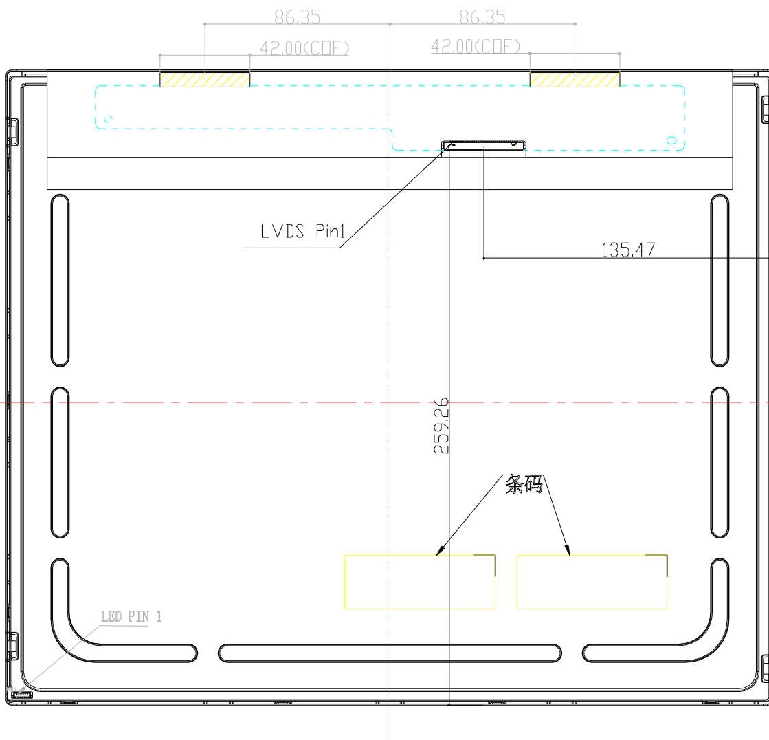
&lt; Figure 5.TFT-LCD Module Outline Dimensions (Rear View) &gt;
