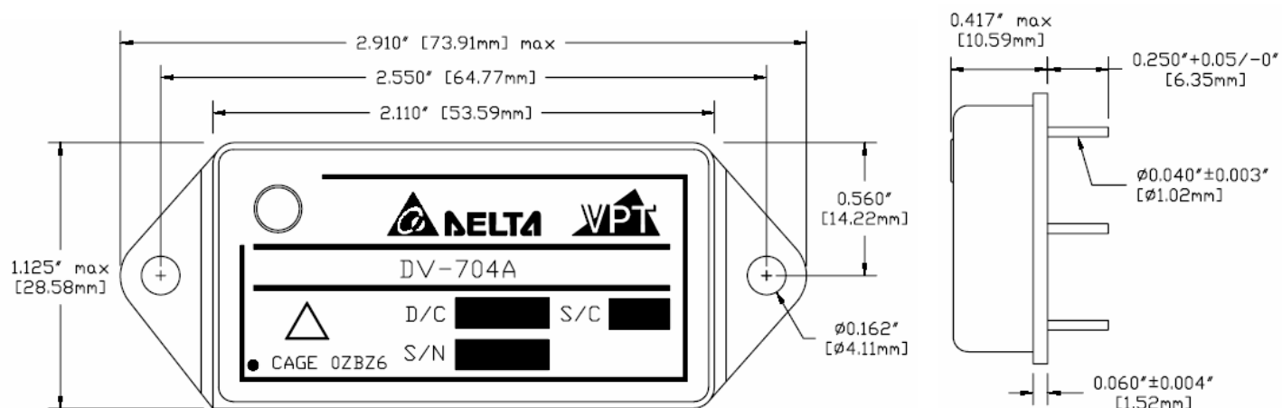
TOP VIEW
