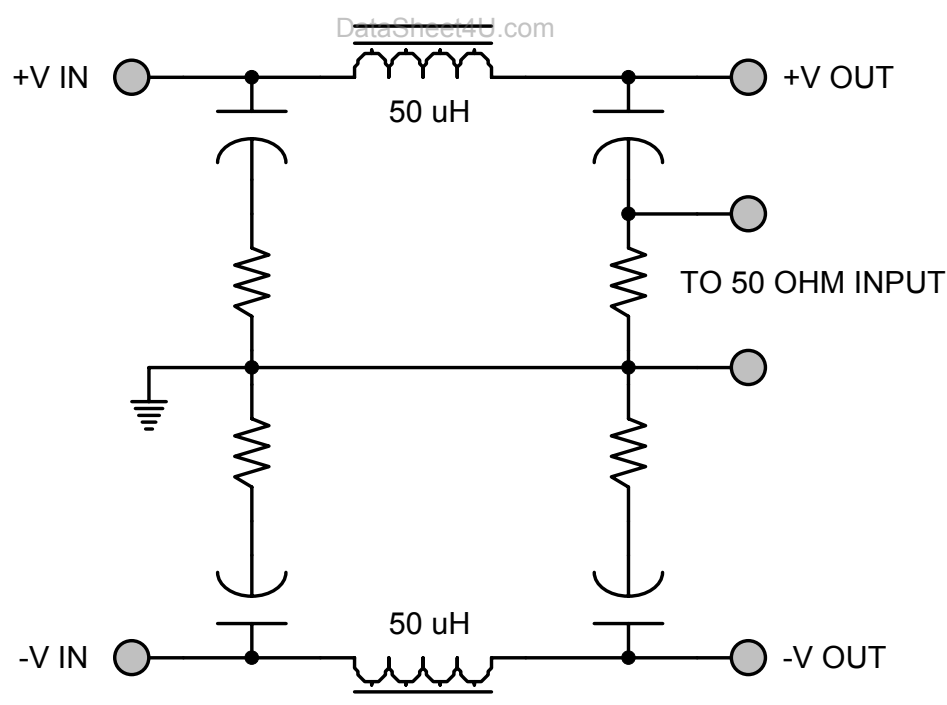
Figure 5 – MIL-STD-461C Measurement Method (Feedthrough Capacitor)
