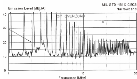
Figure 7 – MIL-STD-461C DVTR2800S Without EMI Filter
